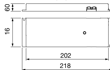
X-Driver 30 W
