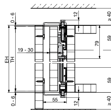
Sistem: HAWA-Concepta 40/50 Conector: Connector 55 mm
