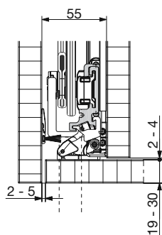
Conector 55 mm Grosime maxima usa: 30 mm
