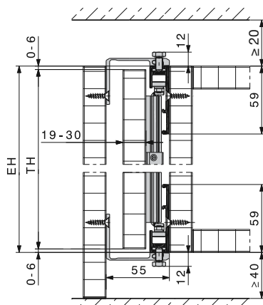
Sistem: HAWA-Concepta 25/30 Conector: Conector 55 mm
