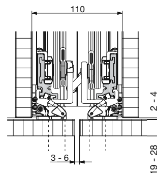
Conector 110 mm Grosime maxima usa: 28 mm
