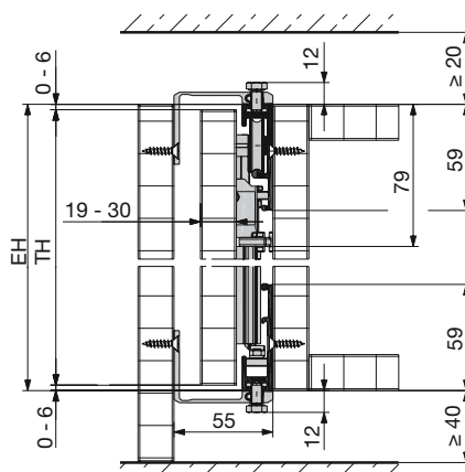
Sistem: HAWA-Concepta 40/50 Conector: Conector 55 mm
