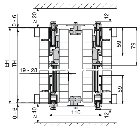
Sistem: HAWA-Concepta 40/50 Conector: Conector 110 mm
