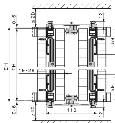
Sistem: HAWA-Concepta 25/30 Conector: Conector 110 mm
