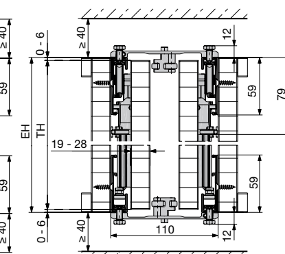
Sistem: HAWA-Concepta 40/50 Conector: Connector 110 mm
