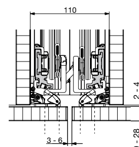
Connector 110 mm Grosime maxima usa: 28 mm
