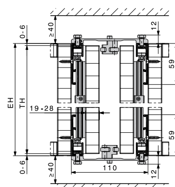
Sistem: HAWA-Concepta 25/30 Conector: Connector 110 mm
