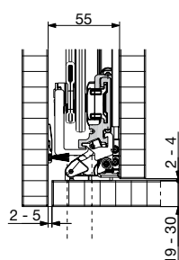
Connector 55 mm Grosime maxima usa: 30 mm
