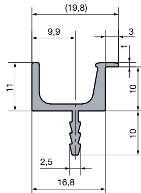
Profil maner cant mobila Grande / Prego eloxat natur
